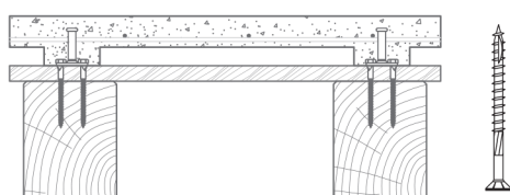
SELF-TAPPING SCREW POWER-FAST FPF-PZ 5,0 x 50 ZPF
