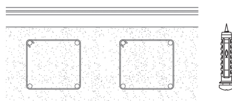
UNIVERSAL WALL PLUG FISCHER SX-SP - 6 x 30 mm (8 x 40 mm)
