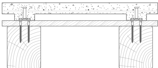
SELF-TAPPING SCREW POWER-FAST FPF-PZ 5,0 X 50 ZPF
